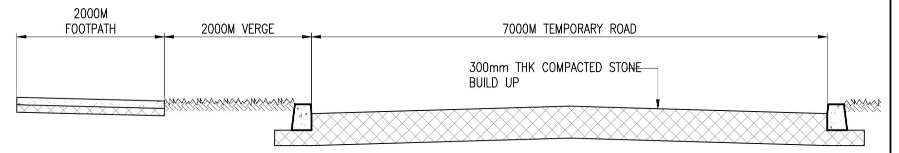
SECTION 2-2 TYPICAL SECTION THROUGH TEMPORARY CONSTRUCTION ACCESS ROAD SCALE 1:50
